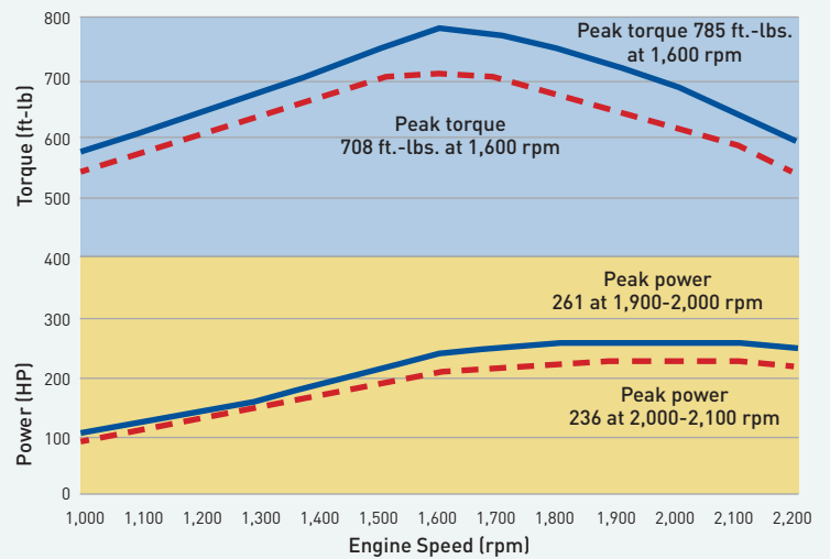
POWER AND TORQUE SR260 (Tier 4) compared to SR240/H8080 (Tier 3)
